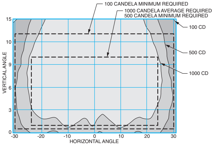
L-852G Runway Guard Light-Yellow
