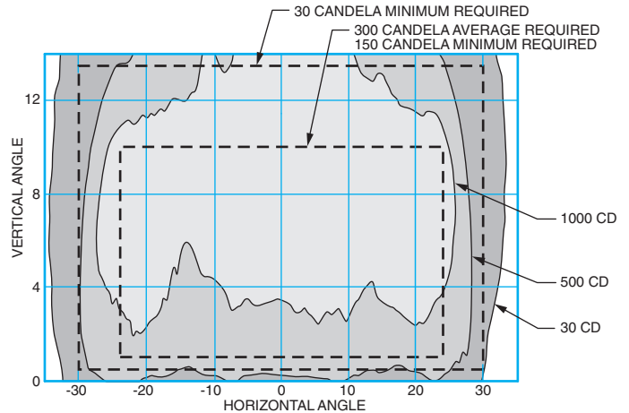
L-852S Stop Bar Light-Red
