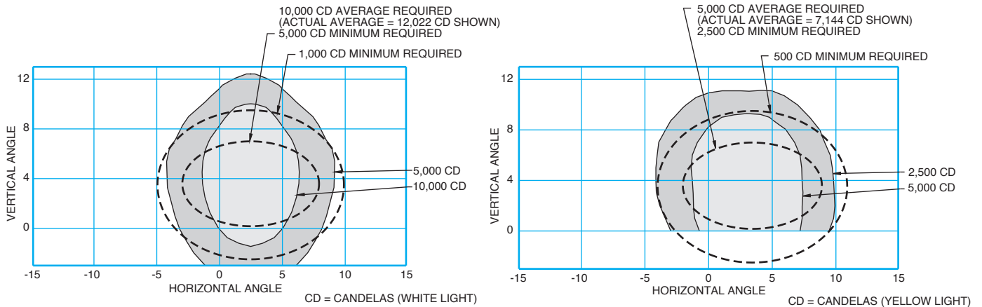
L-850C Inset Runway Edge Light – White
