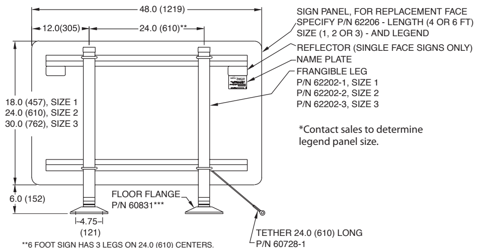
BACK VIEW OF SIGN (4 FOOT SIZE 3 SHOWN)
